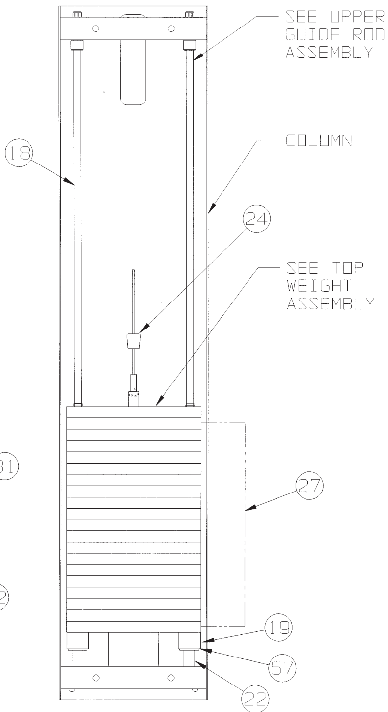
REAR VIEW
