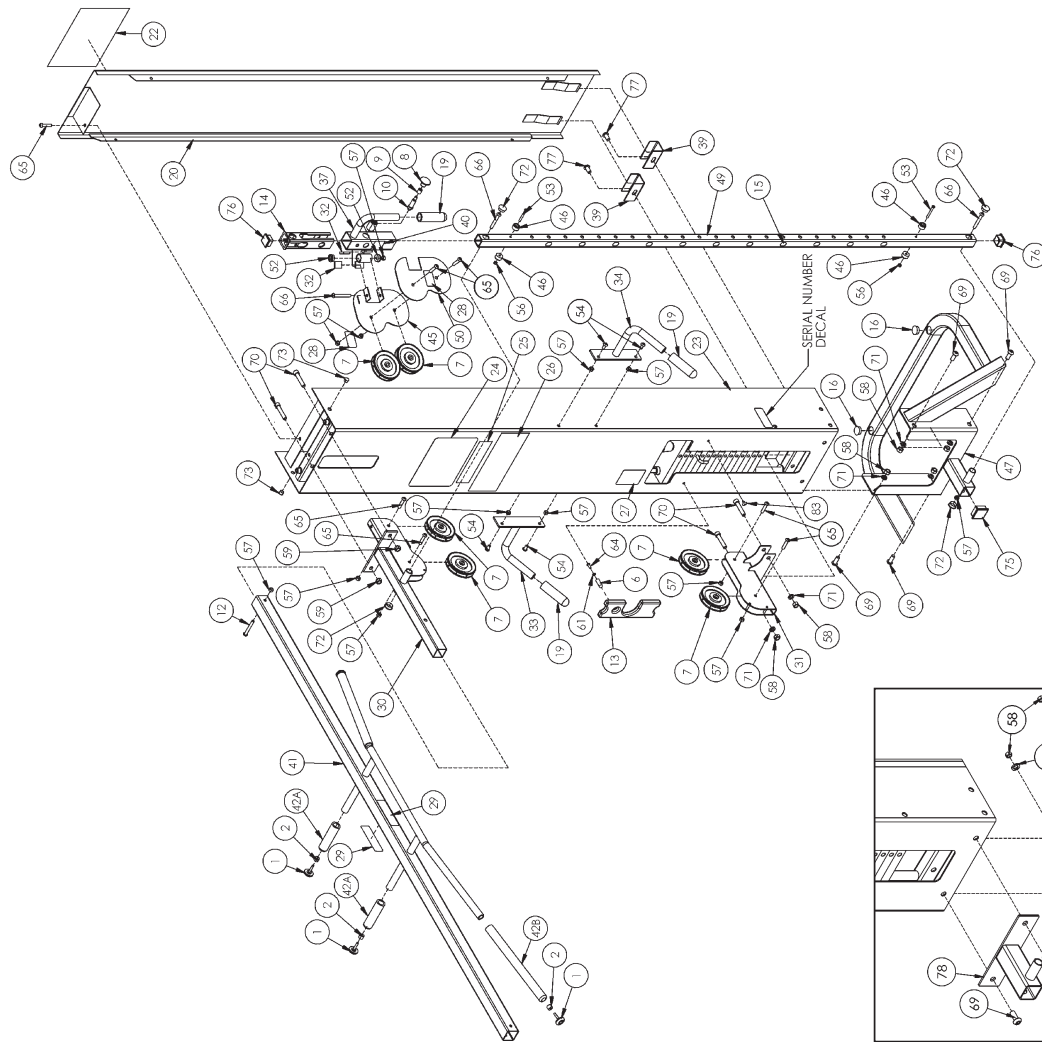
5311 CONFIGURATION
