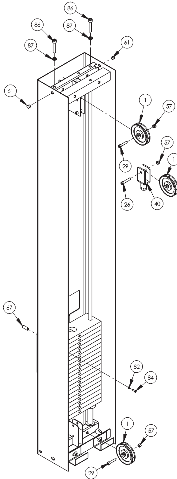
Modular Configuration
